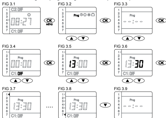
FIG. 3. Programar maniobra de apagado de lunes a viernes a las 13:30 en C1 / Switching OFF programming from Monday to Friday at 13:30 in C1
