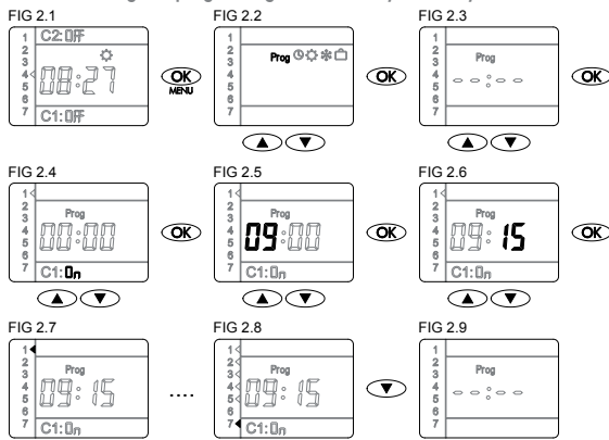
FIG. 2. Programar maniobra de encendido de lunes a viernes a las 09:15 en C1 / Switching ON programming from Monday to Friday at 09:15 in C1
