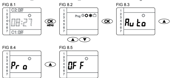
FIG. 8. Cambio horario verano_invierno - invierno_verano / Winter_summer - summer_winter official time change
