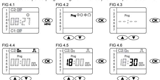
FIG. 4. Programar pulso de 15 seg. a las 18:30 de lunes a viernes en C2 / 15 sec. pulse programing from Monday to Friday at 18:30 in C2
