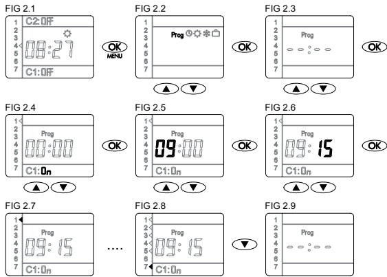
FIG. 2. Programar maniobra de encendido de lunes a viernes a las 09:15 en C1 / Switching ON programing from Monday to Friday at 09:15 in C1
