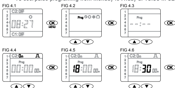
FIG. 4. Programar pulso de 15 seg. a las 18:30 de lunes a viernes en C2 / 15 sec. pulse programming from Monday to Friday at 18:30 in C2
